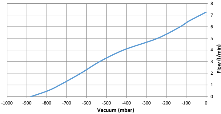
Vacuum / Flow characteristic
